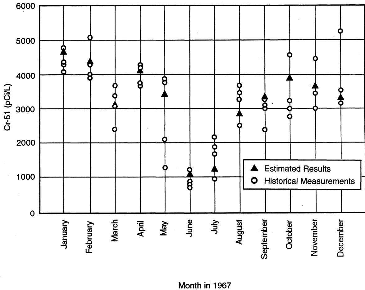
Figure 3.5. Comparison of Estimated versus Measured Radioactivity in Columbia River Water at Richland, Washington (from Walters et al. 1994)
